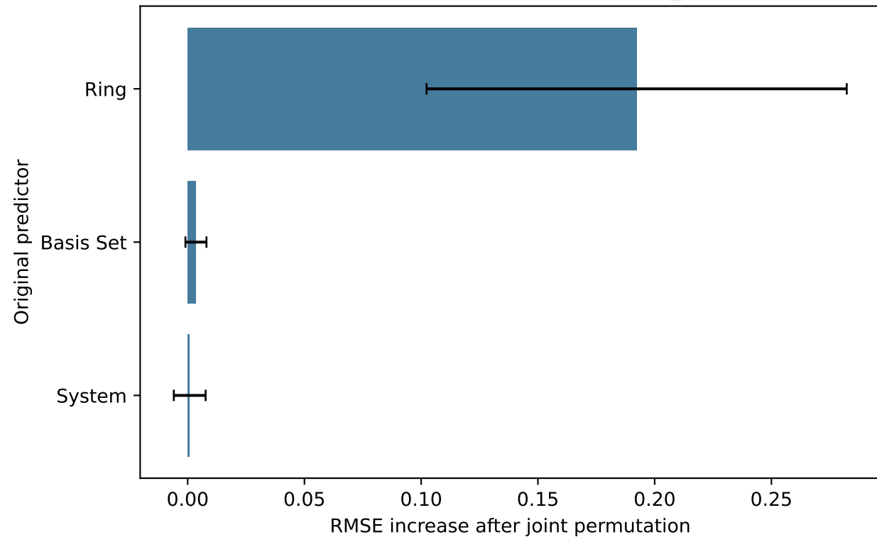
Grouped permutation importance: norm, Q2_(zz-ring atoms)
